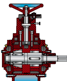
HANDWHEEL
